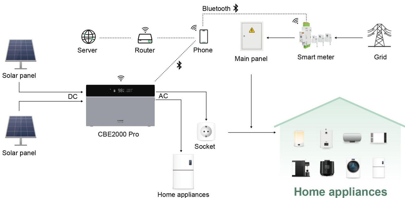
Figure 2-1 Network diagram (New installation)
